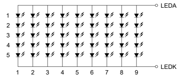
LED Diagram Circuit
